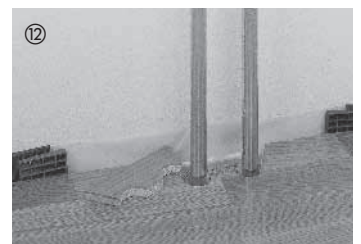
If radiator pipes protrude from the floor, drill and saw a cutout into the board (the size of the cutout depends on the radiator pipe and the required expansion space).
